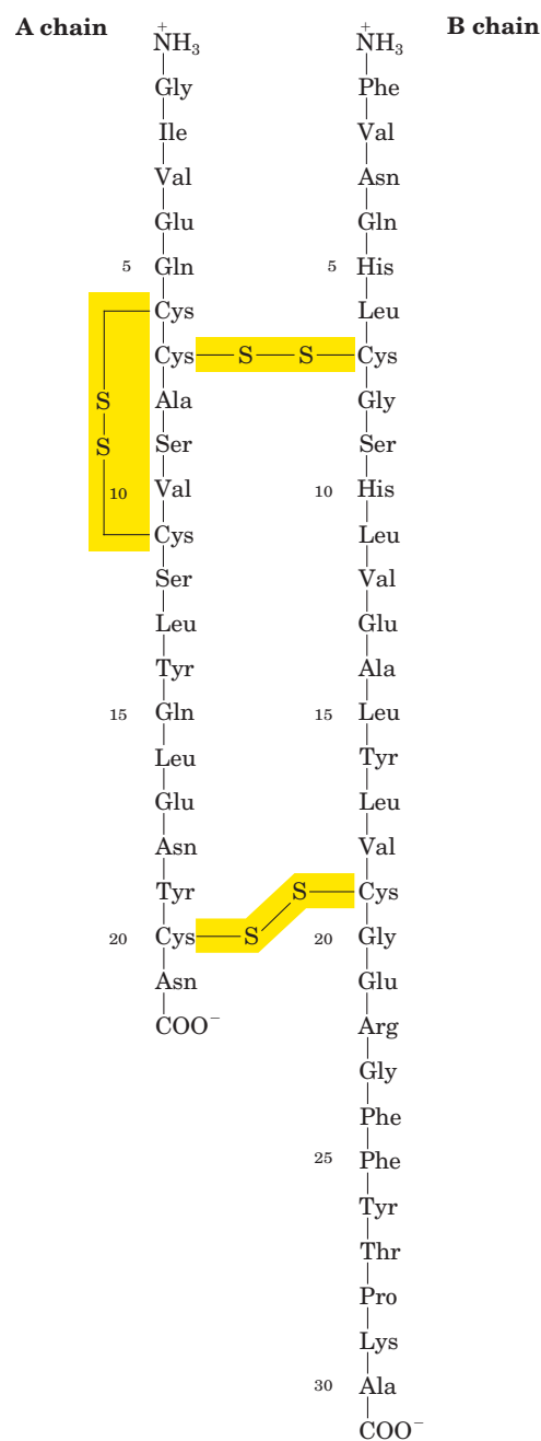
FIGURE 3–24 Amino acid sequence of bovine insulin. The two polypeptide chains are joined by disulfide cross-linkages. The A chain is identical in human, pig, dog, rabbit, and sperm whale insulins. The B chains of the cow, pig, dog, goat, and horse are identical.
