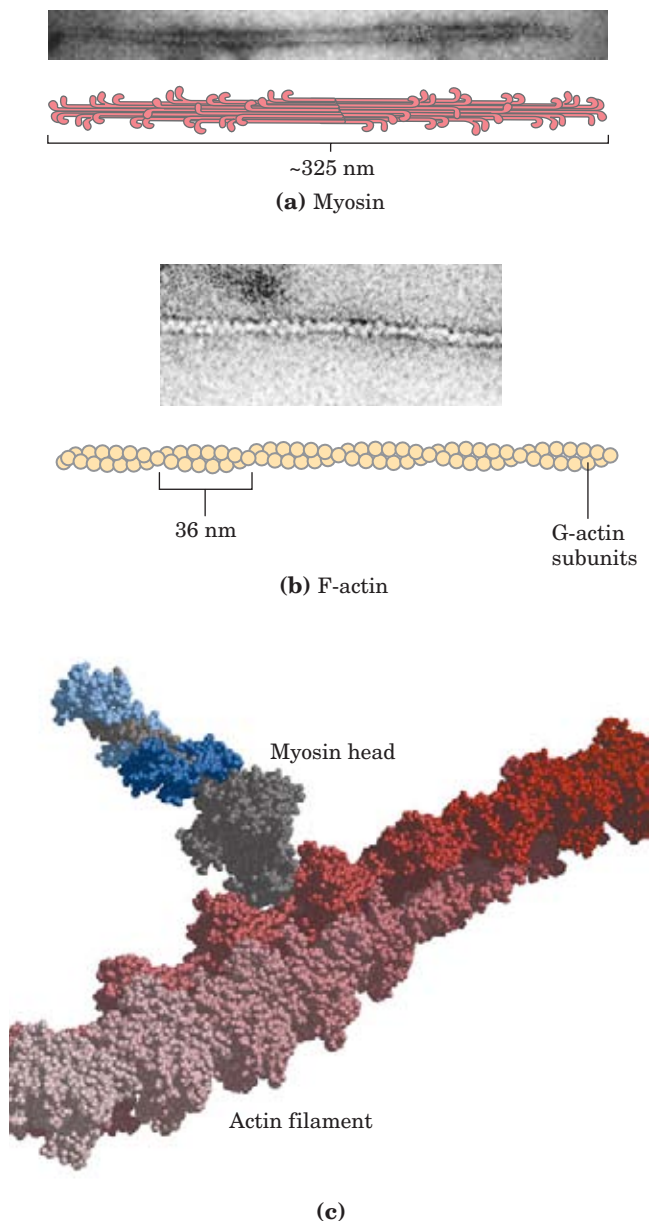
FIGURE 5–28 The major components of muscle. (a) Myosin aggregates to form a bipolar structure called a thick filament. (b) F-actin is a filamentous assemblage of G-actin monomers that polymerize two by two, giving the appearance of two filaments spiraling about one another in a right-handed fashion. (c) Space-filling model of an actin filament (shades of red) with one myosin head (gray and two shades of blue) bound to an actin monomer within the filament (from coordinates supplied by Ivan Rayment).
