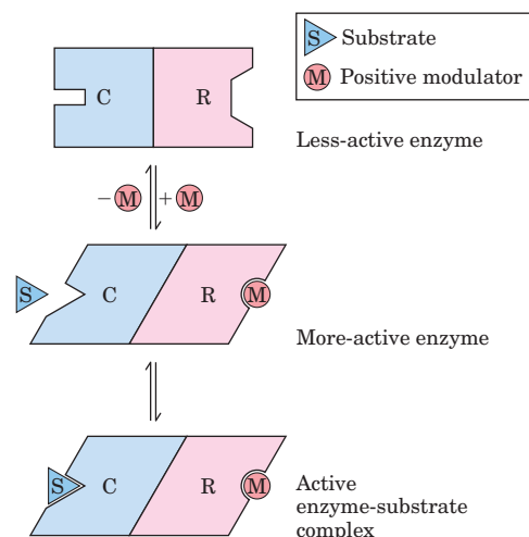
FIGURE 6-31 Subunit interactions in an allosteric enzyme, and interactions with inhibitors and activators. In many allosteric enzymes the substrate binding site and the modulator binding site(s) are on different subunits, the catalytic (C) and regulatory (R) subunits, respectively. Binding of the positive (stimulatory) modulator (M) to its specific site on the regulatory subunit is communicated to the catalytic subunit through a conformational change. This change renders the catalytic subunit active and capable of binding the substrate (S) with higher affinity. On dissociation of the modulator from the regulatory subunit, the enzyme reverts to its inactive or less active form.
