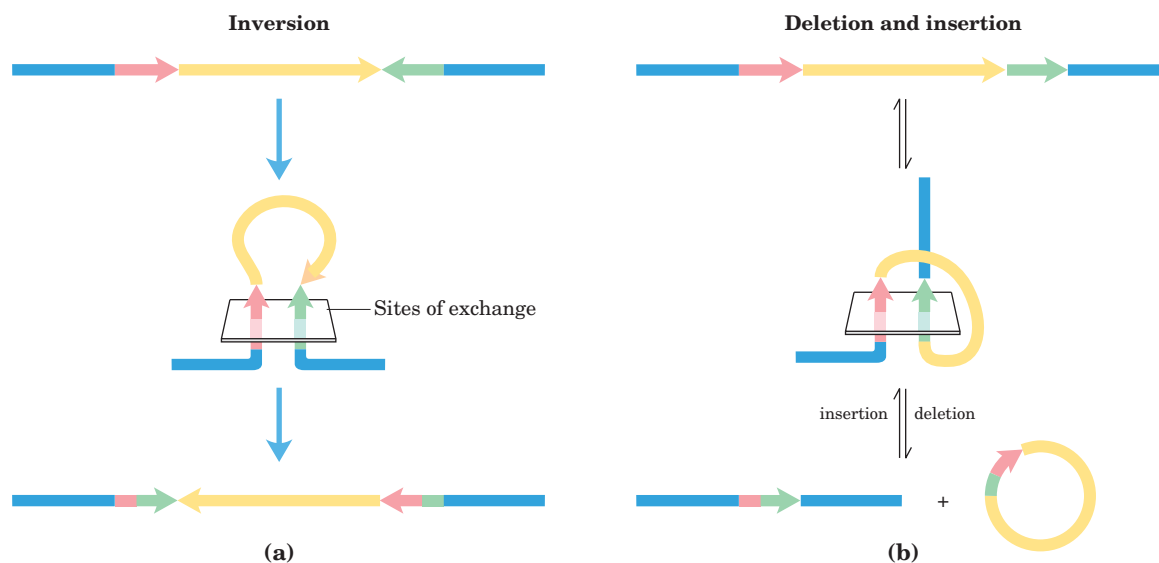
FIGURE 25-41 Effects of site-specific recombination. The outcome of site-specific recombination depends on the location and orientation of the recombination sites (red and green) in a double-stranded DNA molecule. Orientation here (shown by arrowheads) refers to the order of nucleotides in the recombination site, not the 5'→3' direction.
