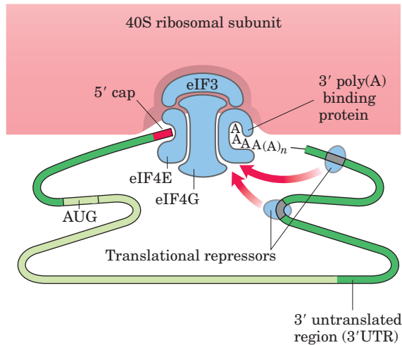
FIGURE 28–35 Translational regulation of eukaryotic mRNA. One of the most important mechanisms for translational regulation in eukaryotes involves the binding of translational repressors (RNA-binding proteins) to specific sites in the 3' untranslated region (3'UTR) of the mRNA. These proteins interact with eukaryotic initiation factors or with the ribosome (see Fig. 27–27) to prevent or slow translation.
