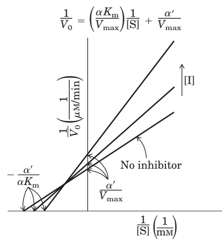
FIGURE 3 Mixed inhibition.
