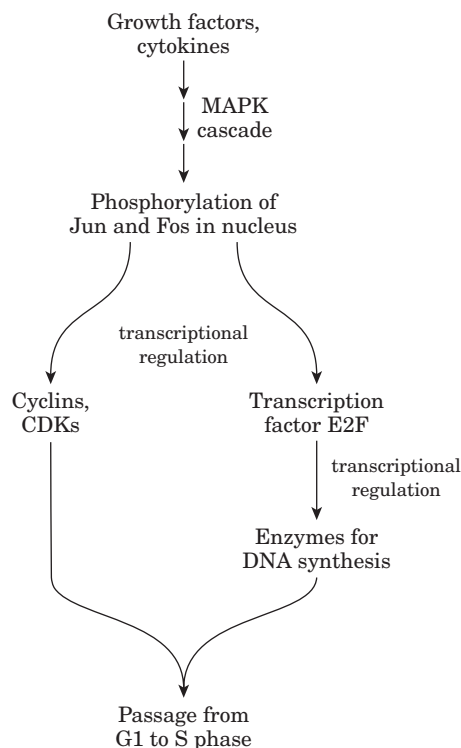
FIGURE 12–47 Regulation of cell division by growth factors. The path from growth factors to cell division leads through the enzyme cascade that activates MAPK; phosphorylation of the nuclear transcription factors Jun and Fos; and the activity of the transcription factor E2F, which promotes synthesis of several enzymes essential for DNA synthesis.
