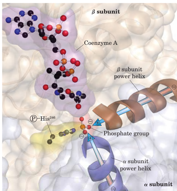
FIGURE 16-12 The succinyl-CoA synthetase reaction. (a) In step ① a phosphoryl group replaces the CoA of succinyl-CoA bound to the enzyme, forming a high-energy acyl phosphate. In step ② the succinyl phosphate donates its phosphoryl group to a His residue of the enzyme, forming a high-energy phosphohistidyl enzyme. In step ③ the phosphoryl group is transferred from the His residue to the terminal phosphate of GDP (or ADP), forming GTP (or ATP). (b) Active site of succinyl-CoA synthetase of E. coli (derived from PDB ID 1SCU). The active site includes part of both the \alpha (blue) and the \beta (brown) subunits. The power helices (blue, brown) place the partial positive charges of the helix dipole near the phosphate group of (P)-His 246 in the \alpha chain, stabilizing the phosphohistidyl enzyme. The bacterial and mammalian enzymes have similar amino acid sequences and three-dimensional structures.
