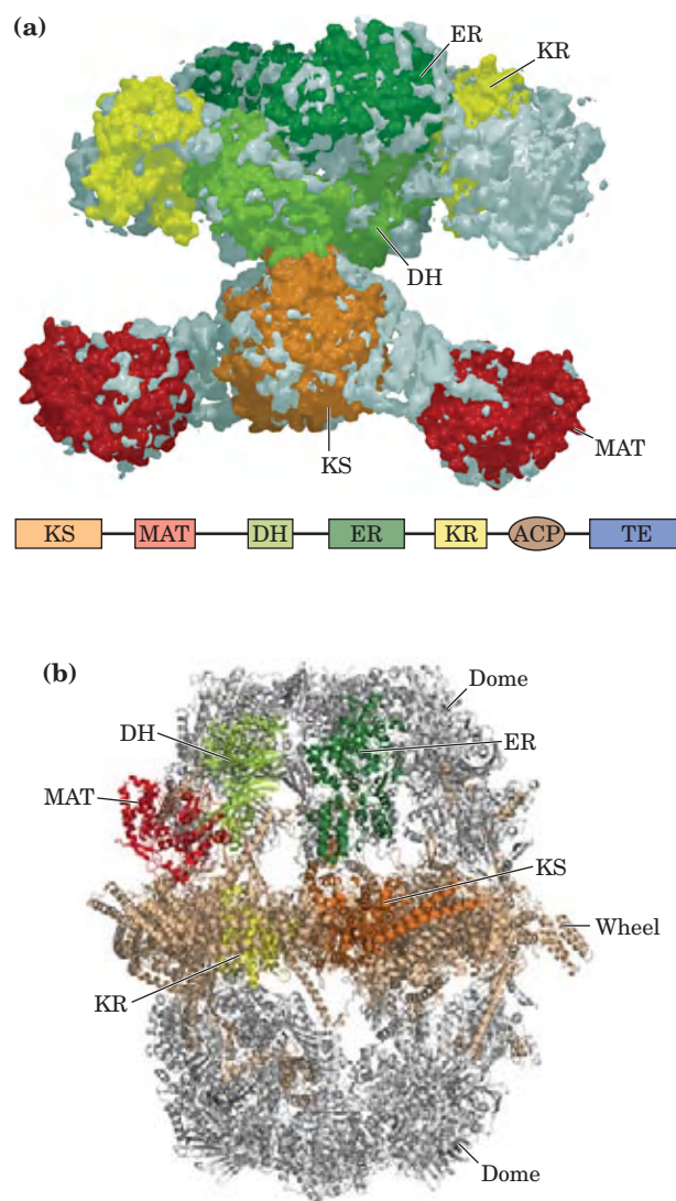
FIGURE 21-3 The structure of fatty acid synthase type I systems. The low-resolution structures of (a) the mammalian (porcine; derived from PDB ID 2CF2) and (b) fungal enzyme systems (derived from PDB IDs 2UV9, 2UVA, 2UVB, and 2UVC) are shown. (a) All of the active sites in the mammalian system are located in different domains within a single large polypeptide chain. The different enzymatic activities are: \beta -ketoacyl-ACP synthase (KS), malonyl/acetyl-CoA-ACP transferase (MAT), \beta -hydroxyacyl-ACP dehydratase (DH), enoyl-ACP reductase (ER), and \beta -ketoacyl-ACP reductase (KR). ACP is the acyl carrier protein. The linear arrangement of the domains in the polypeptide is shown in the lower panel. The seventh domain (TE) is a thioesterase that releases the palmitate product from ACP when the synthesis is completed. The ACP and TE domains are disordered in the crystal and are therefore not shown in the structure. (b) In the structure of the FAS I from the fungus Thermomyces lanuginosus , the same active sites are divided between two multifunctional polypeptide chains that function together. Six copies of each polypeptide are found in the heterododecameric complex. A wheel of six \alpha subunits, which include ACP as well as the KS and KR active sites, is found at the center of the complex. In the wheel three subunits are found on one face, three on the other. On either side of the wheel are domes formed by trimers of the \beta subunits (containing the ER and DH active sites, as well as two domains with active sites analogous to MAT in the mammalian enzyme). The domains of one of each type of subunit are colored according to the active site colors of the mammalian enzyme in (a).
