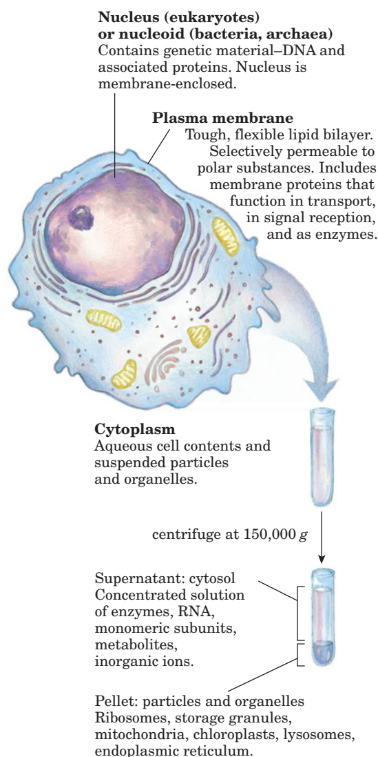
FIGURE 1–3 The universal features of living cells. All cells have a nucleus or nucleoid, a plasma membrane, and cytoplasm. The cytosol is defined as that portion of the cytoplasm that remains in the supernatant after gentle breakage of the plasma membrane and centrifugation of the resulting extract at 150,000 g for 1 hour.
