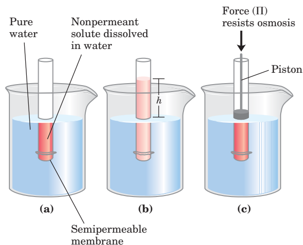
FIGURE 2-11 Osmosis and the measurement of osmotic pressure.
