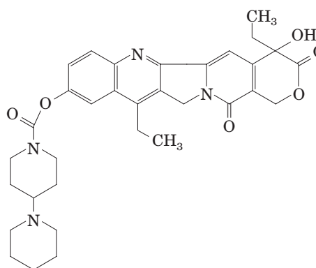
Irinotecan
