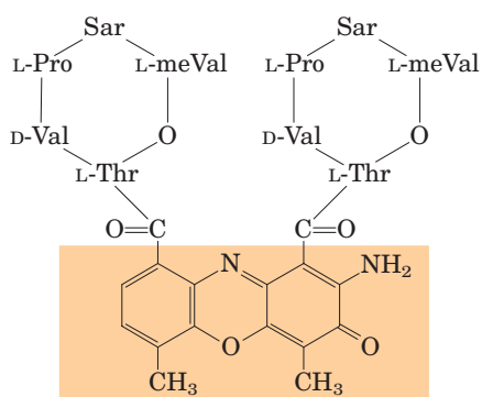
Actinomycin D
