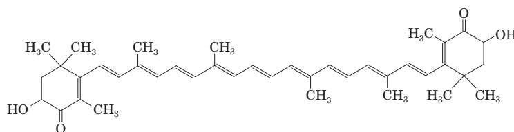
Astaxanthin
