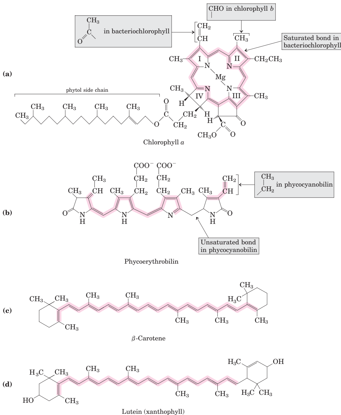
FIGURE 19–47 Primary and secondary photopigments. (a) Chlorophylls a and b and bacteriochlorophyll are the primary gatherers of light energy. (b) Phycoerythrobilin and phycocyanobilin (phycobilins) are the antenna pigments in cyanobacteria and red algae. (c) \beta -
