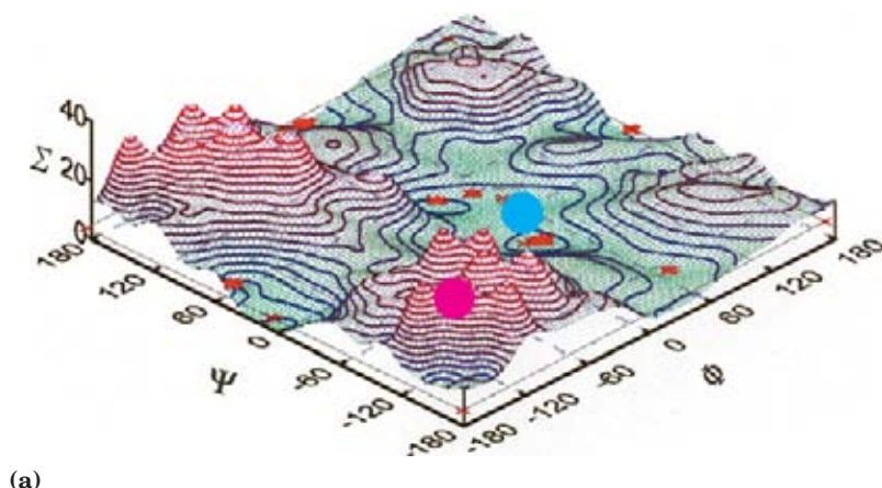
FIGURE 7-19 A map of favored conformations for oligosaccharides and polysaccharides. The torsion angles \Psi and \phi (see Fig. 7-18), which define the spatial relationship between adjacent rings, can in principle have any value from 0^\circ to 360^\circ . In fact, some of the torsion angles would give conformations that are sterically hindered, whereas others give conformations that maximize hydrogen bonding. (a) When the relative energy ( \Sigma ) is plotted for each value of \phi and \Psi , with isoenergy ("same energy") contours drawn at intervals of 1 kcal/mol above the minimum
