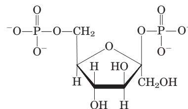
Fructose 2,6-bisphosphate
