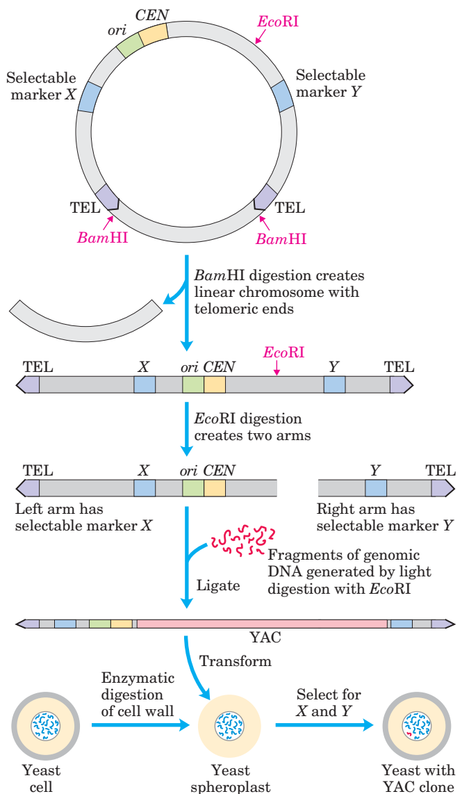
FIGURE 9-7 Construction of a yeast artificial chromosome (YAC). A YAC vector includes an origin of replication ( ori ), a centromere ( CEN ), two telomeres ( TEL ), and selectable markers ( X and Y ). Digestion with Bam HI and Eco RI generates two separate DNA arms, each with a telomeric end and one selectable marker. A large segment of DNA (e.g., up to 2 \times 10^6 bp from the human genome) is ligated to the two arms to create a yeast artificial chromosome. The YAC transforms yeast cells (prepared by removal of the cell wall to form spheroplasts), and the cells are selected for X and Y ; the surviving cells propagate the DNA insert.
