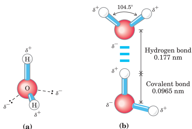
FIGURE 2-1 Structure of the water molecule. (a) The dipolar nature of the H 2 O molecule is shown in a ball-and-stick model; the dashed lines represent the nonbonding orbitals. There is a nearly tetrahedral arrangement of the outer-shell electron pairs around the oxygen atom; the two hydrogen atoms have localized partial positive charges ( \delta^+ ) and the oxygen atom has a partial negative charge ( \delta^- ). (b) Two H 2 O molecules joined by a hydrogen bond (designated here, and throughout this book, by three blue lines) between the oxygen atom of the upper molecule and a hydrogen atom of the lower one. Hydrogen bonds are longer and weaker than covalent O—H bonds.
