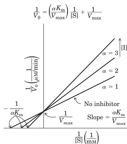
FIGURE 1 Competitive inhibition.
