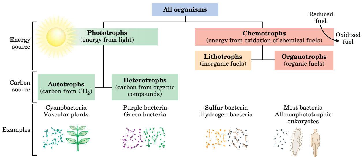
FIGURE 1–5 Organisms can be classified according to their source of energy (sunlight or oxidizable chemical compounds) and their source of carbon for the synthesis of cellular material.
