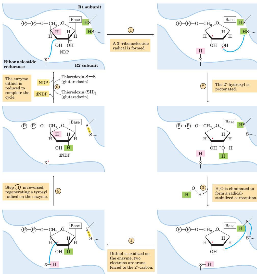
MECHANISM FIGURE 22-41
