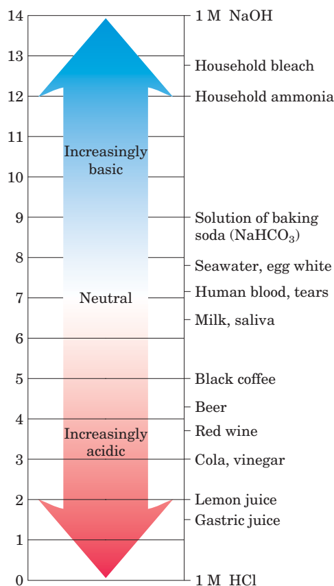
FIGURE 2-14 The pH of some aqueous fluids.
