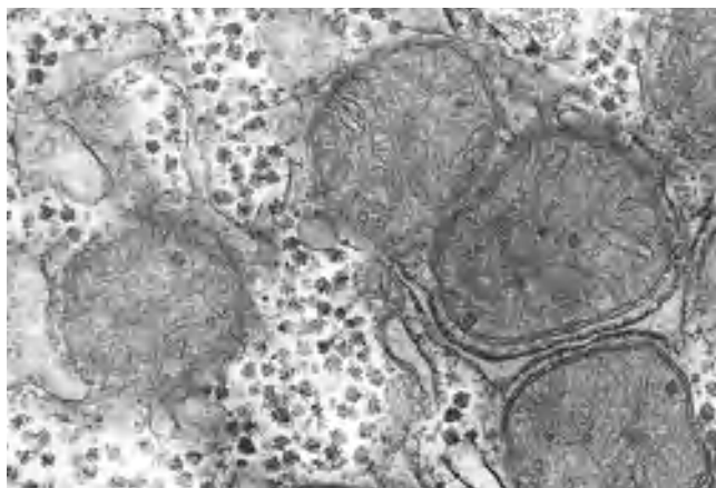
FIGURE 15–24 Glycogen granules in a hepatocyte. Glycogen, a storage form of carbohydrate, appears as electron-dense particles, often in aggregates or rosettes. In hepatocytes glycogen is closely associated with tubules of the smooth endoplasmic reticulum. Many mitochondria are also evident in this micrograph.
