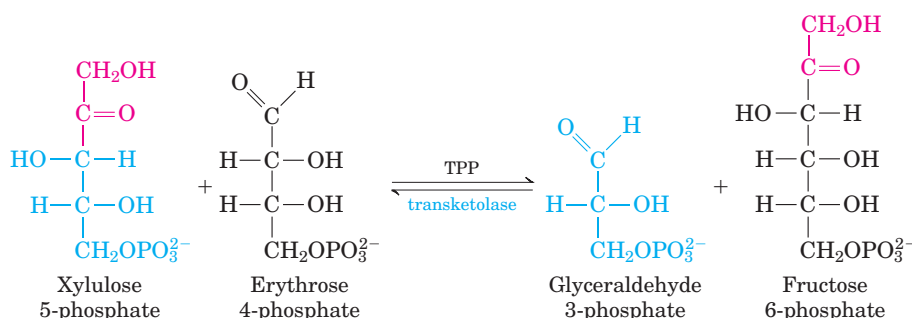
(a) Transketolase
